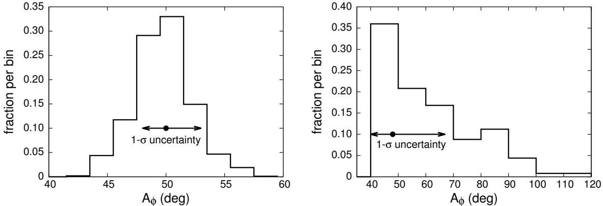
Fig. 15.— Distributions of A_\phi for two plutinos. The left panel shows OSSOS plutino o3o15, where the A_\phi distribution is nearly symmetric around the best-fit orbit’s A_\phi . The right panel shows o3o20PD, which has a very asymmetric A_\phi distribution. In both panels the best-fit orbit’s A_\phi is indicated by a black circle and the arrows show what we are calling the 1\sigma uncertainties.
