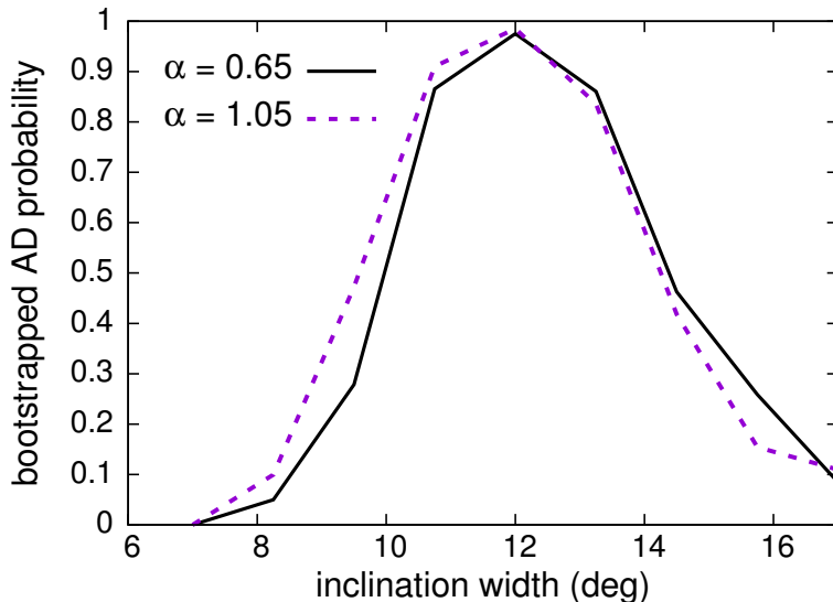
Fig. 3.— The bootstrapped AD probability of various values of the inclination width \sigma_i for two different H distributions. The rejectable range of \sigma_i (AD probability below 0.05) does not change much when comparing two very different H distributions.
