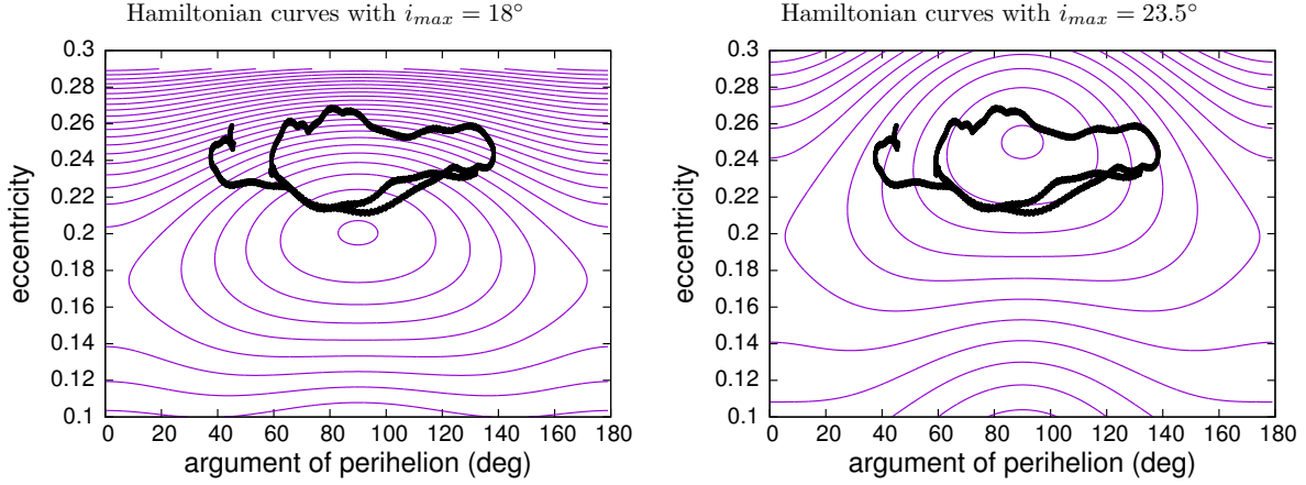
Fig. 18.— Evolution of plutino o3o08 (black dots) from a numerical simulation that includes the Sun and the four outer planets plotted over approximate Hamiltonian level curves for i_{max} = 18^\circ (left panel) and i_{max} = 23.5^\circ (right panel). The object has i_{max} = 18^\circ , but the poor match in the left panel indicates that the expression for the approximate Hamiltonian in the three body problem as given by Wan & Huang (2007) is not a good match to the dynamics in the full integrations.
